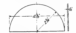
BEARING BORE-GAUGE 4 1/2 x 8 JOURNAL
